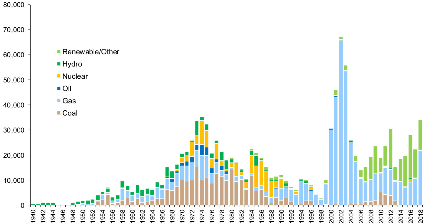
U.S. Electric Generating Capacity by In Service Year: 1940 – 2018 (Nameplate Capacity; MW)
